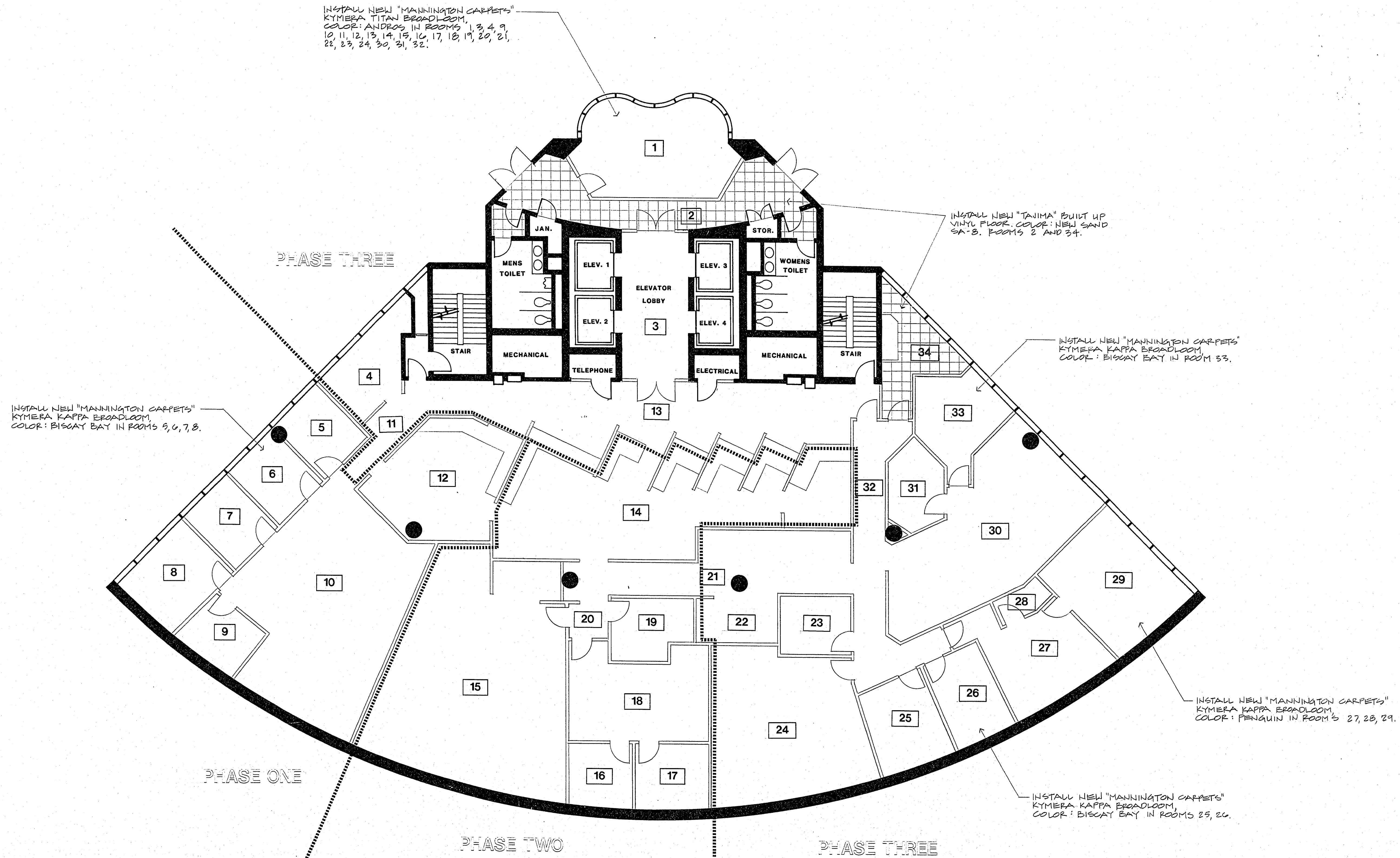
CARPET AND TILE PLAN 1/8" = 1'-0"
