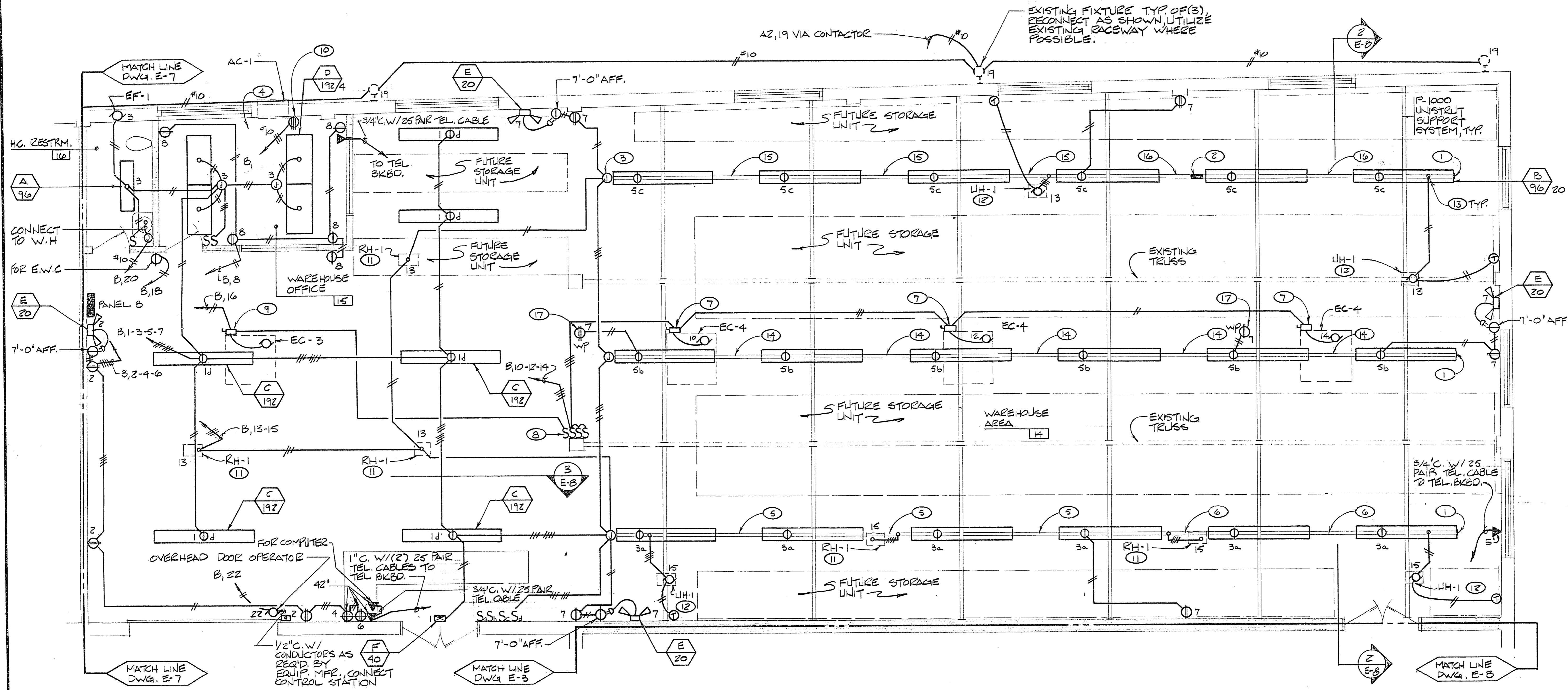
PARTIAL 1 ST FLOOR PLAN - LIGHTING & POWER. SCALE: 1/4" = 1'-0"
