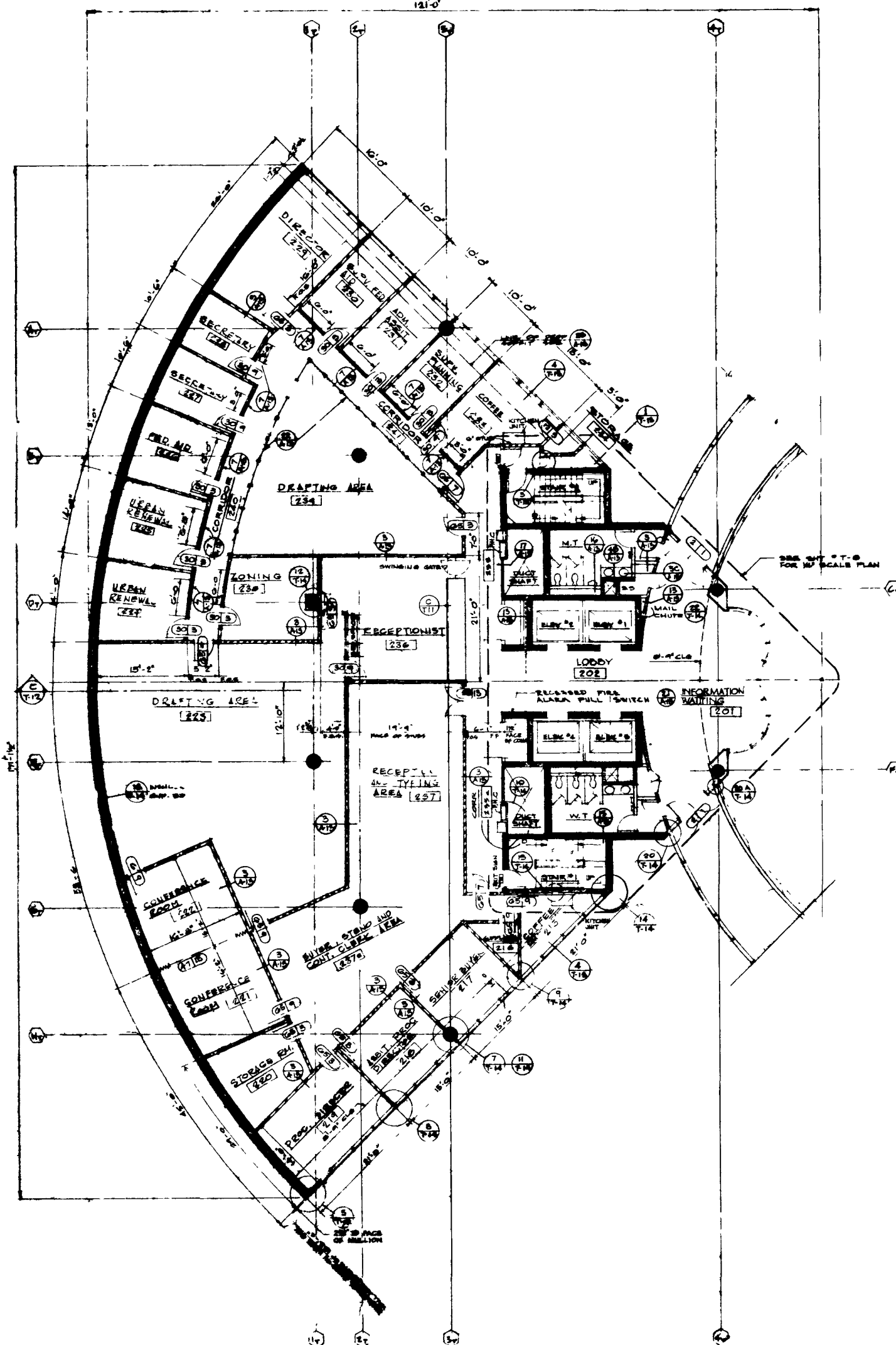
2 ND FLOOR
