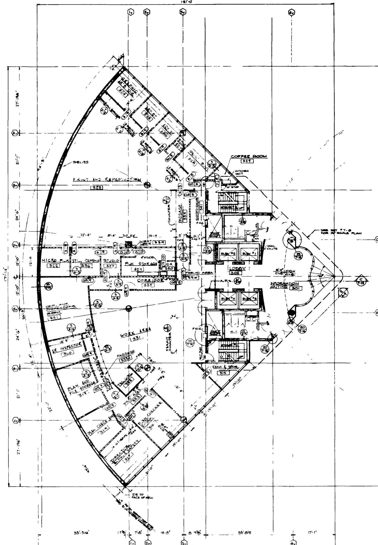
3 RD FLOOR
