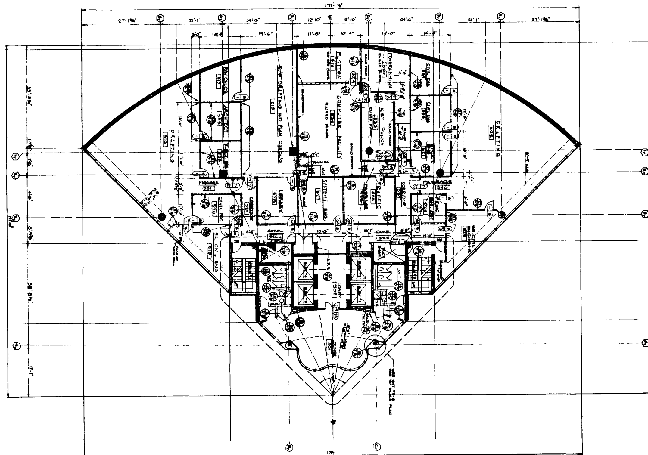
5 TH FLOOR
