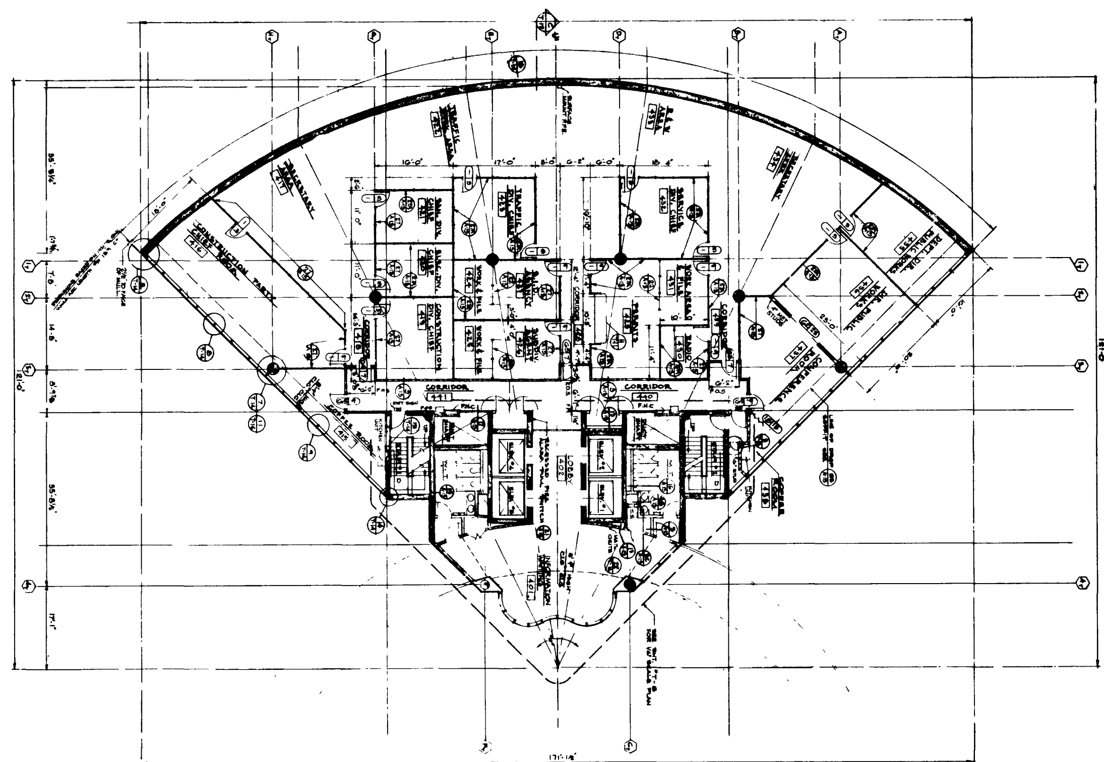
4 TH FLOOR
