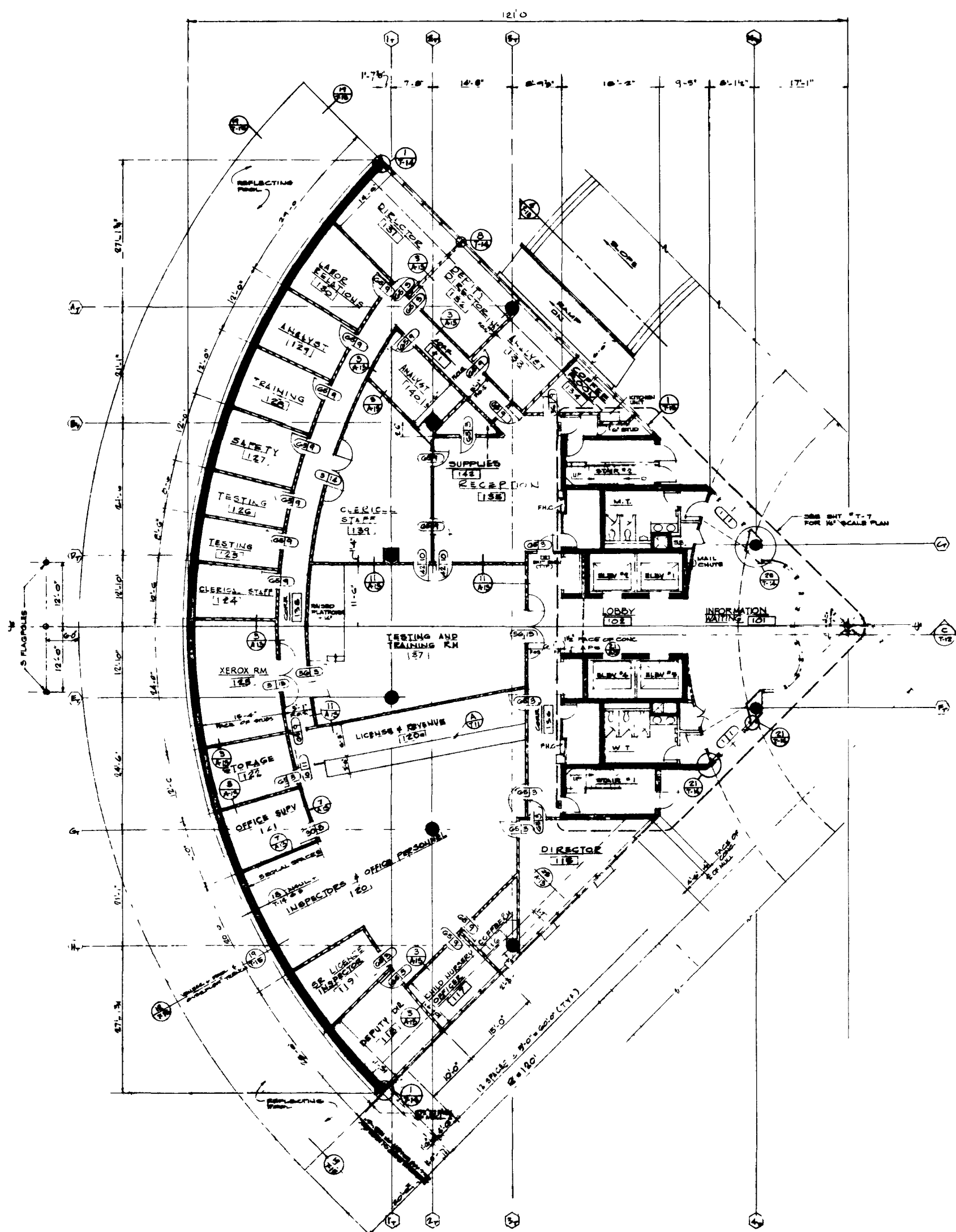
PLAZA LEVEL FLOOR PLAN
