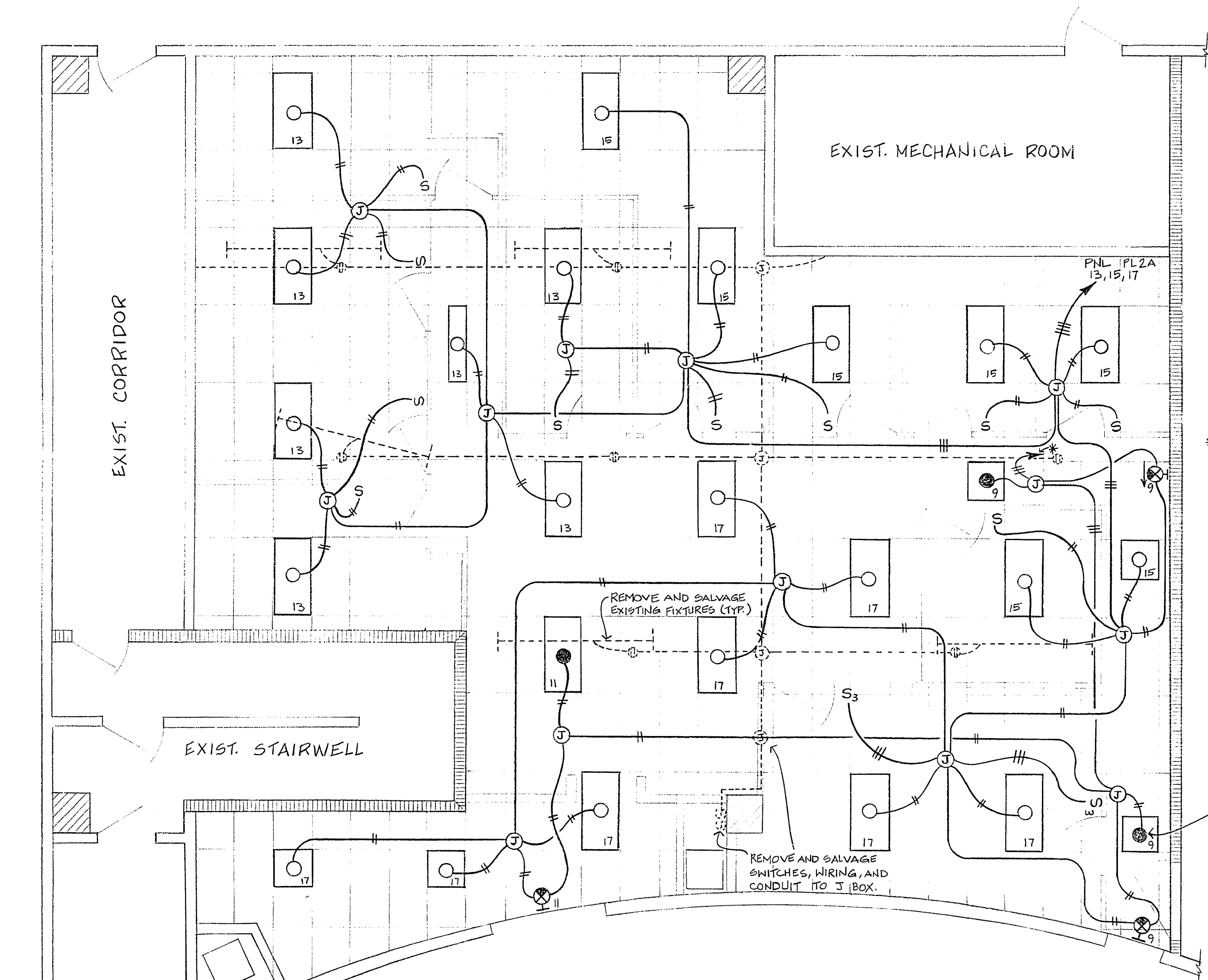
LIGHTING PLAN REFLECTED CEILING VIEW 1/4" = 1'-0"
