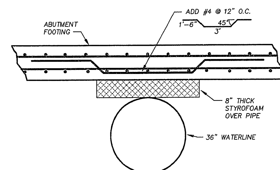
ABUTMENT FTG. OVER WATERLINE
