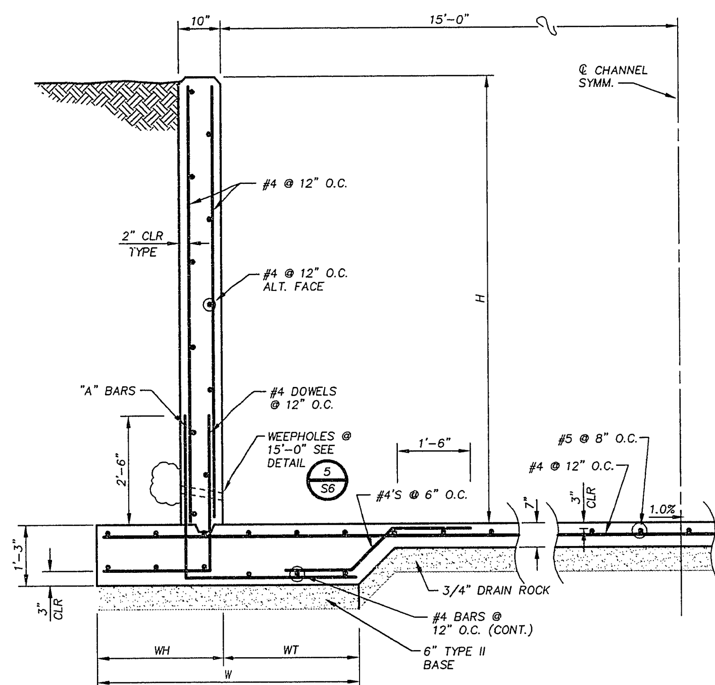
CHANNEL SECTION
