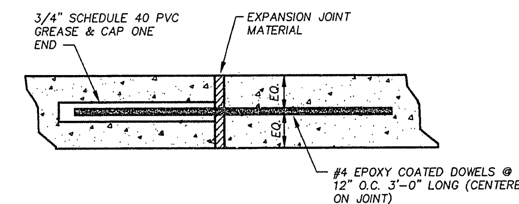
DOWELED EXPANSION JOINT
