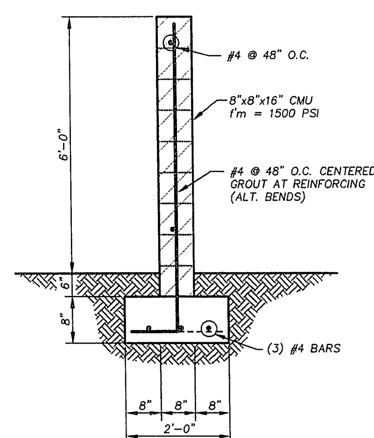
CMU WALL
