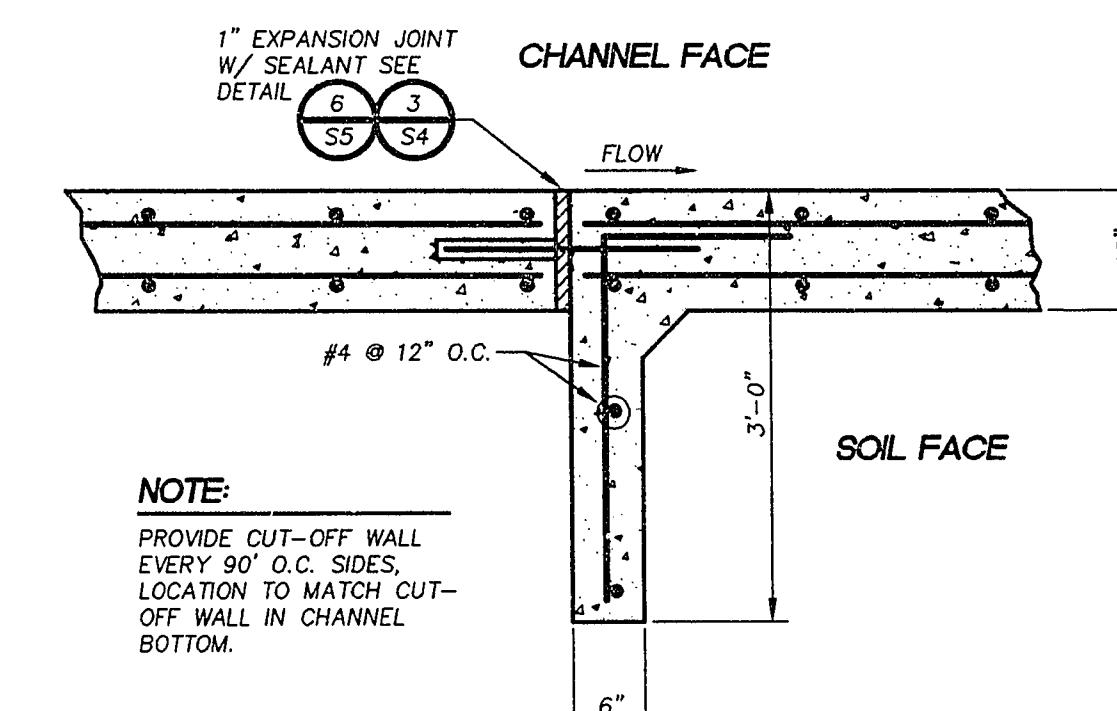
SECTION CUT-OFF WALL
