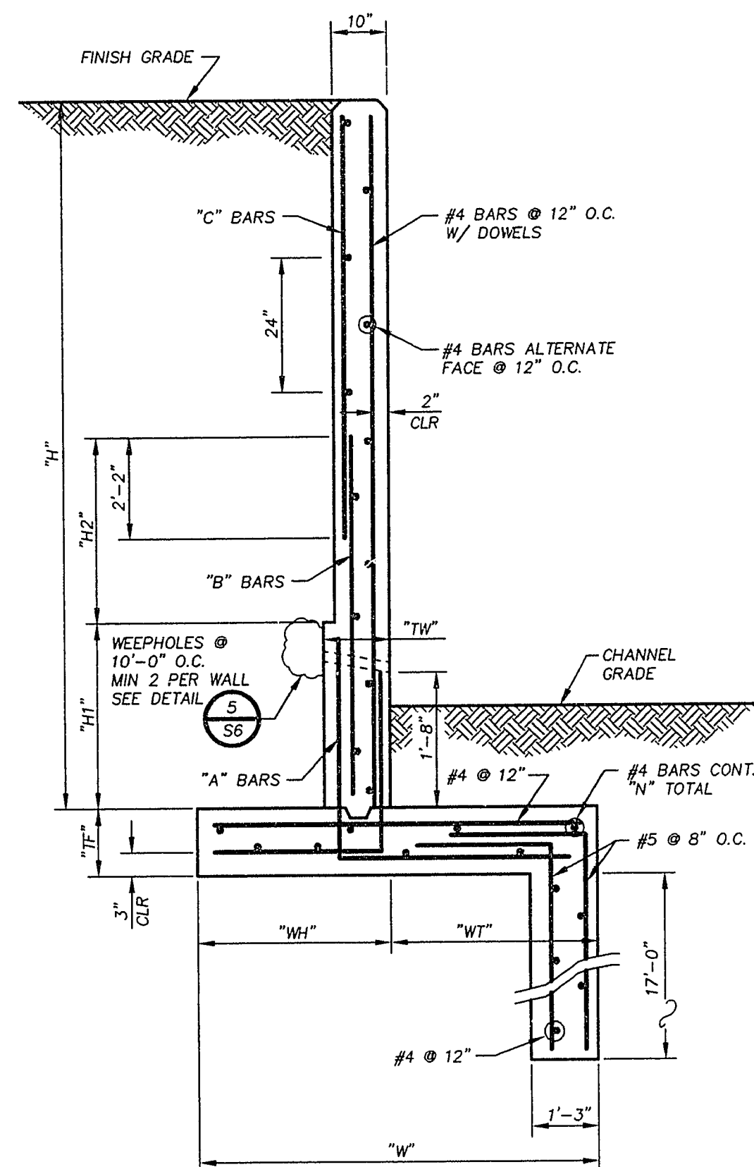
HEADWALL SECTION
