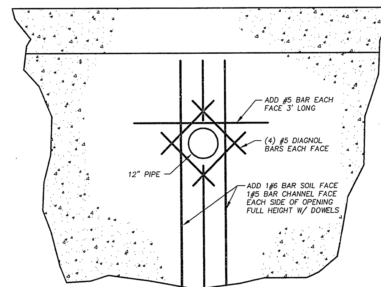
12" PIPE OPENING DETAIL
