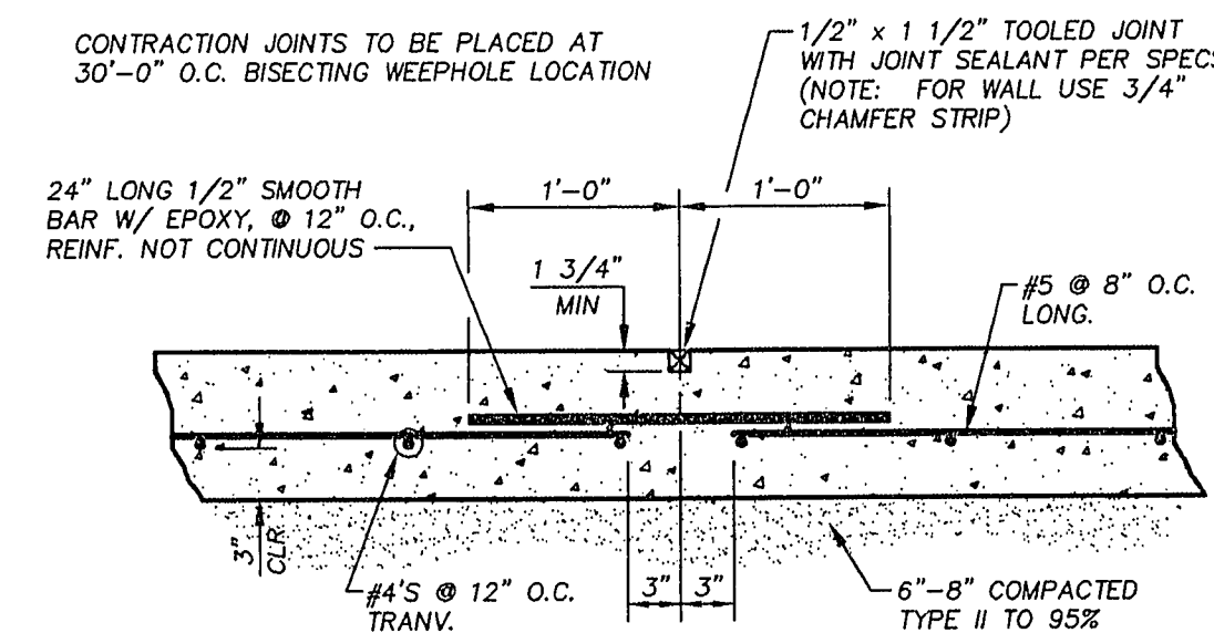
TYPICAL CONTRACTION JOINT DETAIL
