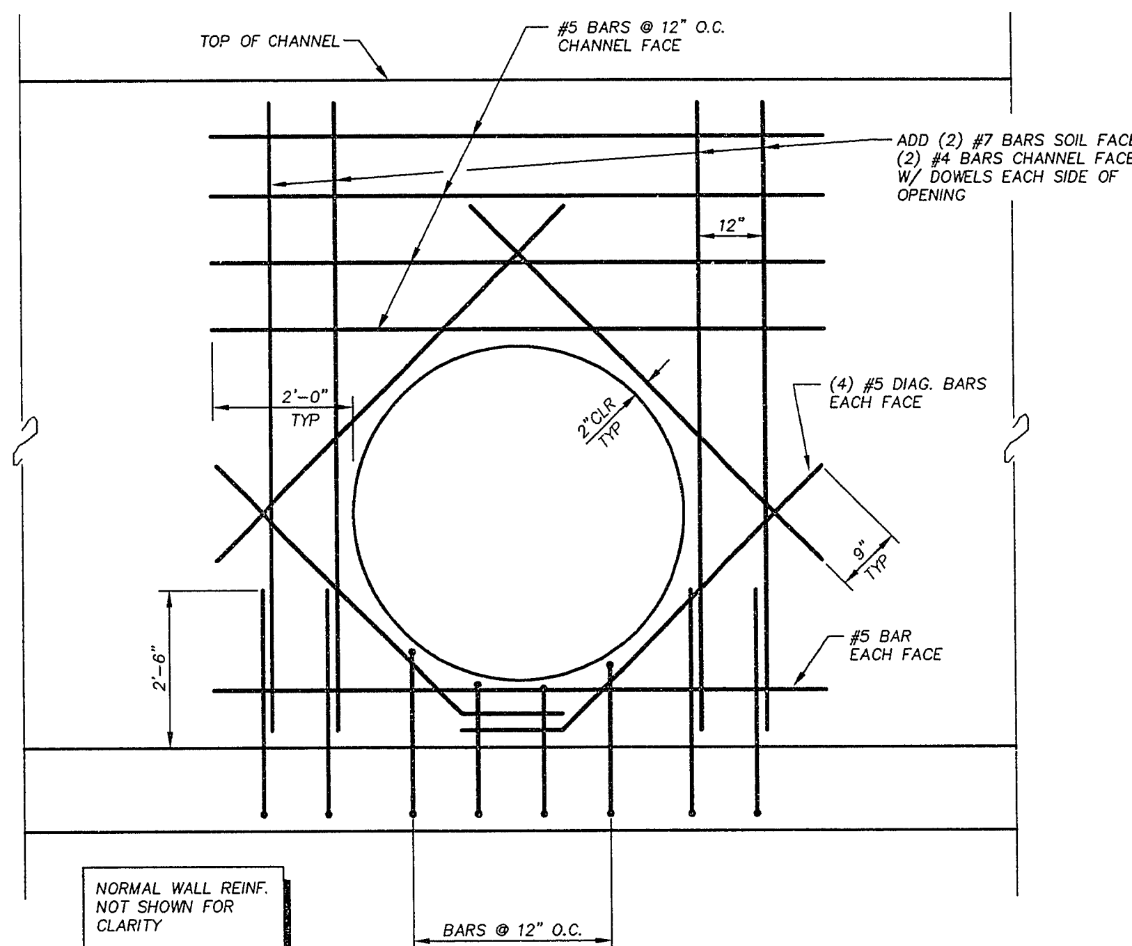
TYPICAL PIPE OPENING DETAIL
