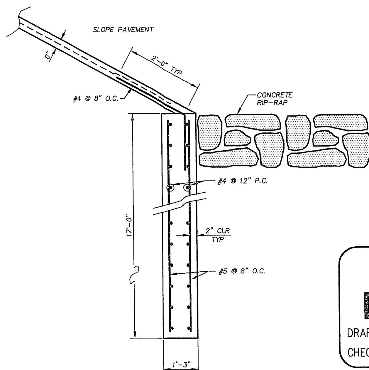
CUT-OFF WALL DETAIL
