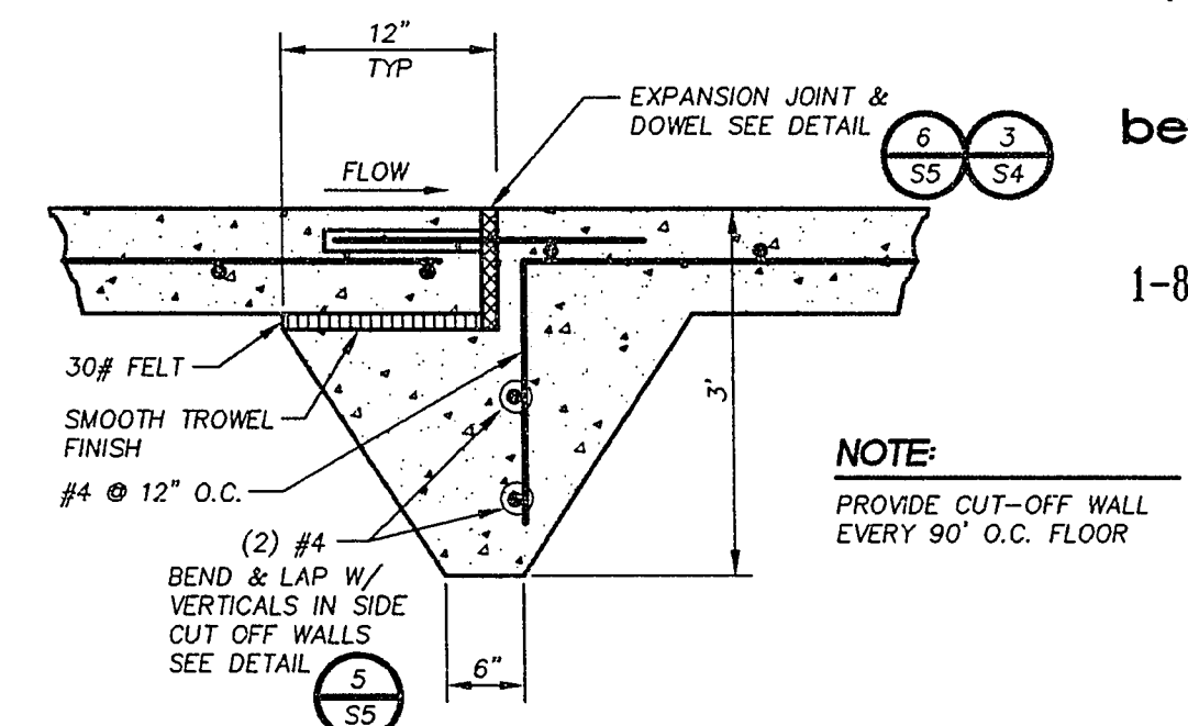
SECTION CUT-OFF WALL
