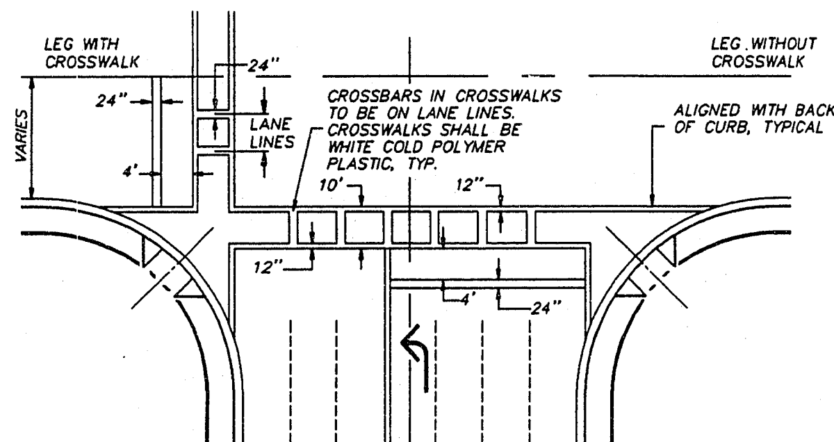
TYPICAL CROSSWALK / STOP BAR DETAIL
