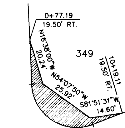
SVRE DETAIL '3' NOT TO SCALE
