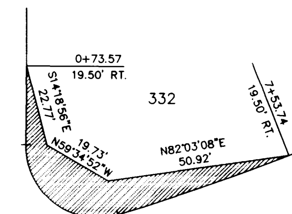
SVRE DETAIL '5' NOT TO SCALE
