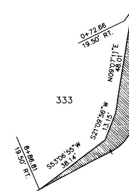
SVRE DETAIL '4' NOT TO SCALE
