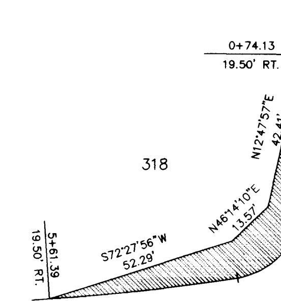
SVRE DETAIL '6' NOT TO SCALE
