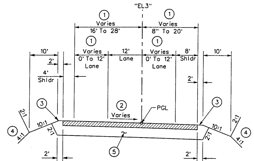
"EL3" SECTION OF IMPROVEMENT "EL3" 154+0.00 To "EL3" 157+55.63
