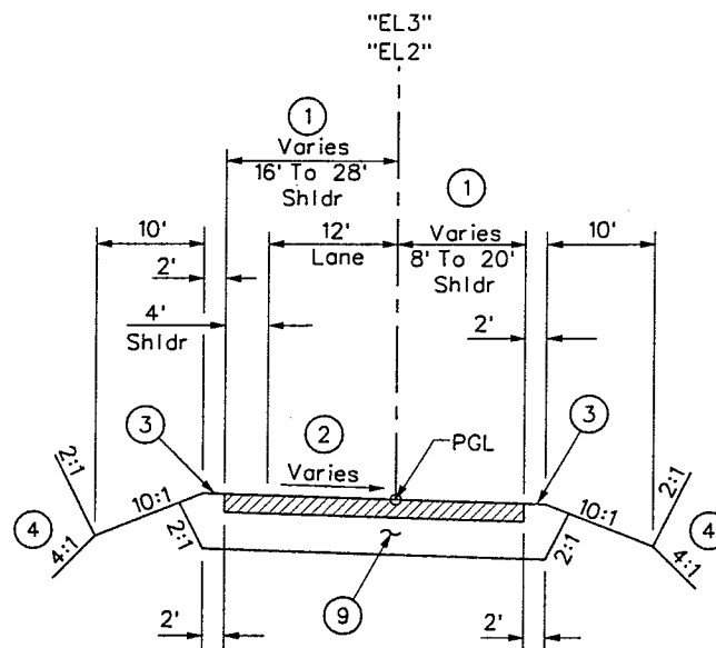
"EL2", "EL3" SECTION OF IMPROVEMENT "EL2" 60+23.69 To "EL2" 65+00.00 "EL3" 139+44.18 To "EL3" 154+00.00
