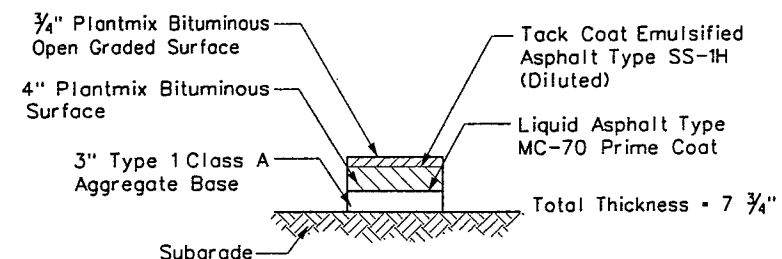
PAVEMENT STRUCTURAL SECTION NO 4 NTS
