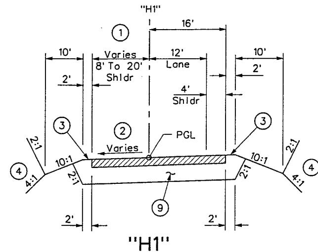
SECTION OF IMPROVEMENT "H1" 84+22.91 To "H1" 88+00.00
