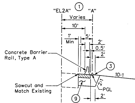
"EL2A" SECTION OF IMPROVEMENT "EL2A" 82+05.92 To "EL2A" 84+05.67
