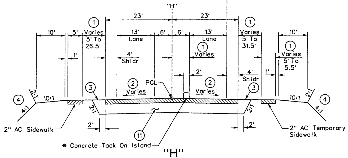
SECTION OF IMPROVEMENT
