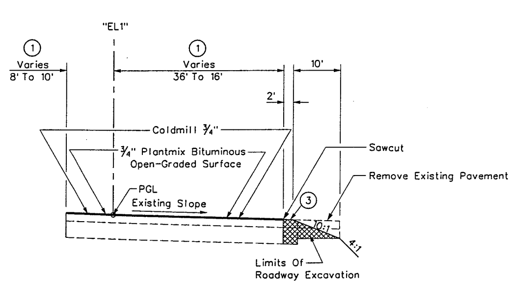
"EL1" SECTION OF IMPROVEMENT "EL1" 58+00.36 To "EL1" 69+29.867
