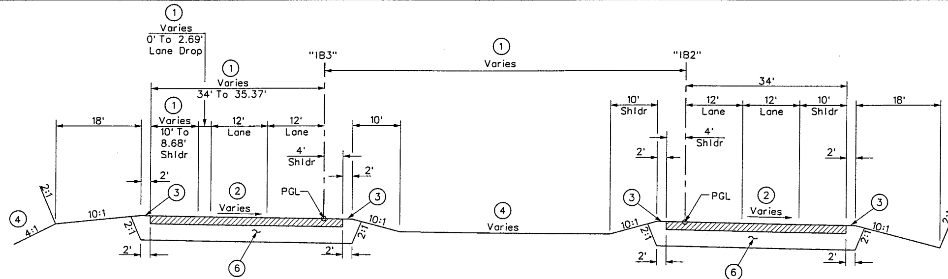
"IB3" SECTION OF IMPROVEMENT
