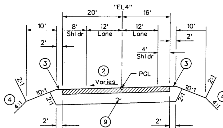
"EL4" SECTION OF IMPROVEMENT "EL4" 152+00.00 To "EL4" 156+31.10
