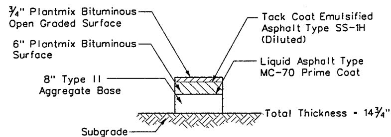
PAVEMENT STRUCTURAL SECTION NO 2 NTS
