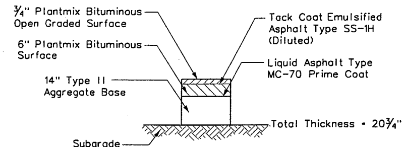
PAVEMENT STRUCTURAL SECTION NO 7 NTS
