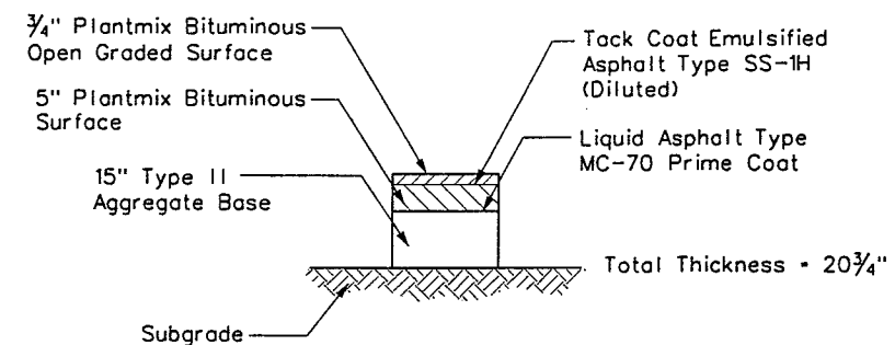
PAVEMENT STRUCTURAL SECTION NO 5 NTS
