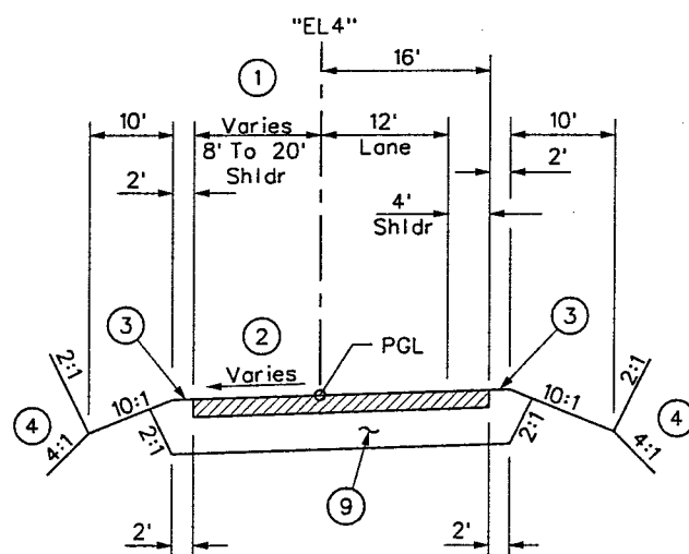
"EL4" SECTION OF IMPROVEMENT "EL4" 142+03.23 To "EL4" 152+00.00
