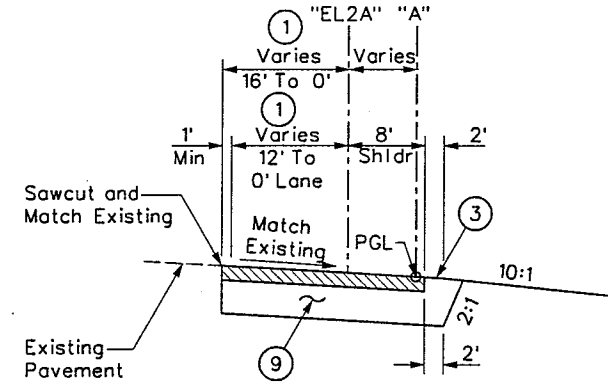
"EL2A" SECTION OF IMPROVEMENT "EL2A" 75+12.46 To "EL2A" 82+05.92
