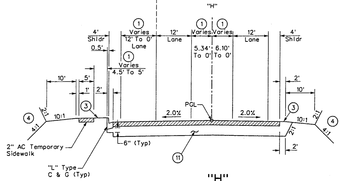
SECTION OF IMPROVEMENT
