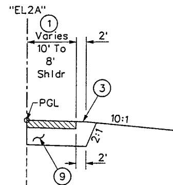
"EL2A" SECTION OF IMPROVEMENT "EL2A" 71+00.00 To "EL2A" 75+12.46 Rt
