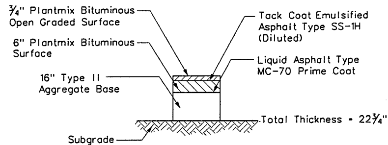
PAVEMENT STRUCTURAL SECTION NO 1 NTS
