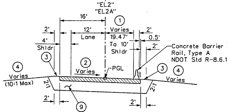
"EL2", "EL2A" SECTION OF IMPROVEMENT "EL2" 65+00.00 To "EL2" 69+56.78 "EL2A" 69+56.78 To "EL2A" 71+00.00 Rt "EL2A" 69+56.78 To "EL2A" 75+12.46 Lt
