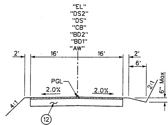
"AW" "BD1" "BD2" "CB" "DS" "DS2" "EL" SECTION OF IMPROVEMENT "AW" 100+00.00 To "AW" 106+68.43 "BD1" 100+00.00 To "BD1" 106+78.05 "BD2" 150+16.00 To "BD2" 189+86.83 "CB" 100+00.000 To "CB" 106+61.67 "DS" 80+00.65 To "DS" 126+68.82 "DS2" 100+00.00 To "DS2" 113+34.95 "EL" 30+45.00 To "EL" 36+37.47
