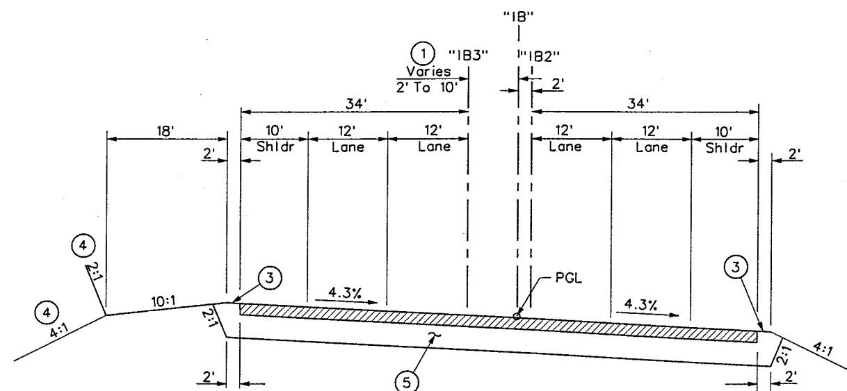
"IB" SECTION OF IMPROVEMENT
