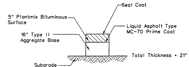
PAVEMENT STRUCTURAL SECTION NO 8 NTS
