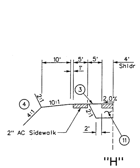
SECTION OF IMPROVEMENT
