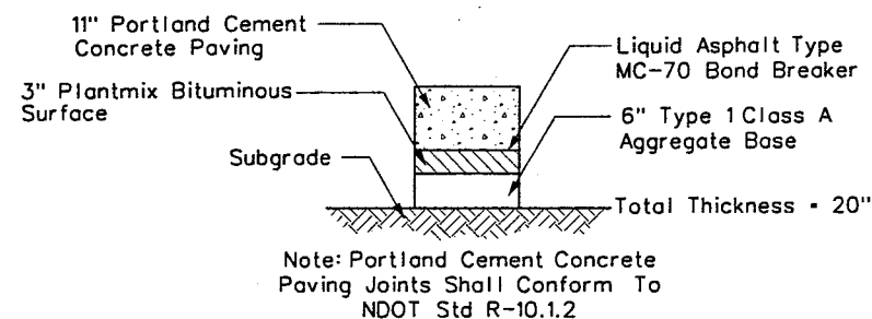
PAVEMENT STRUCTURAL SECTION NO 3 NTS
