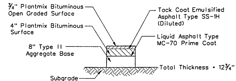
PAVEMENT STRUCTURAL SECTION NO 6 NTS
