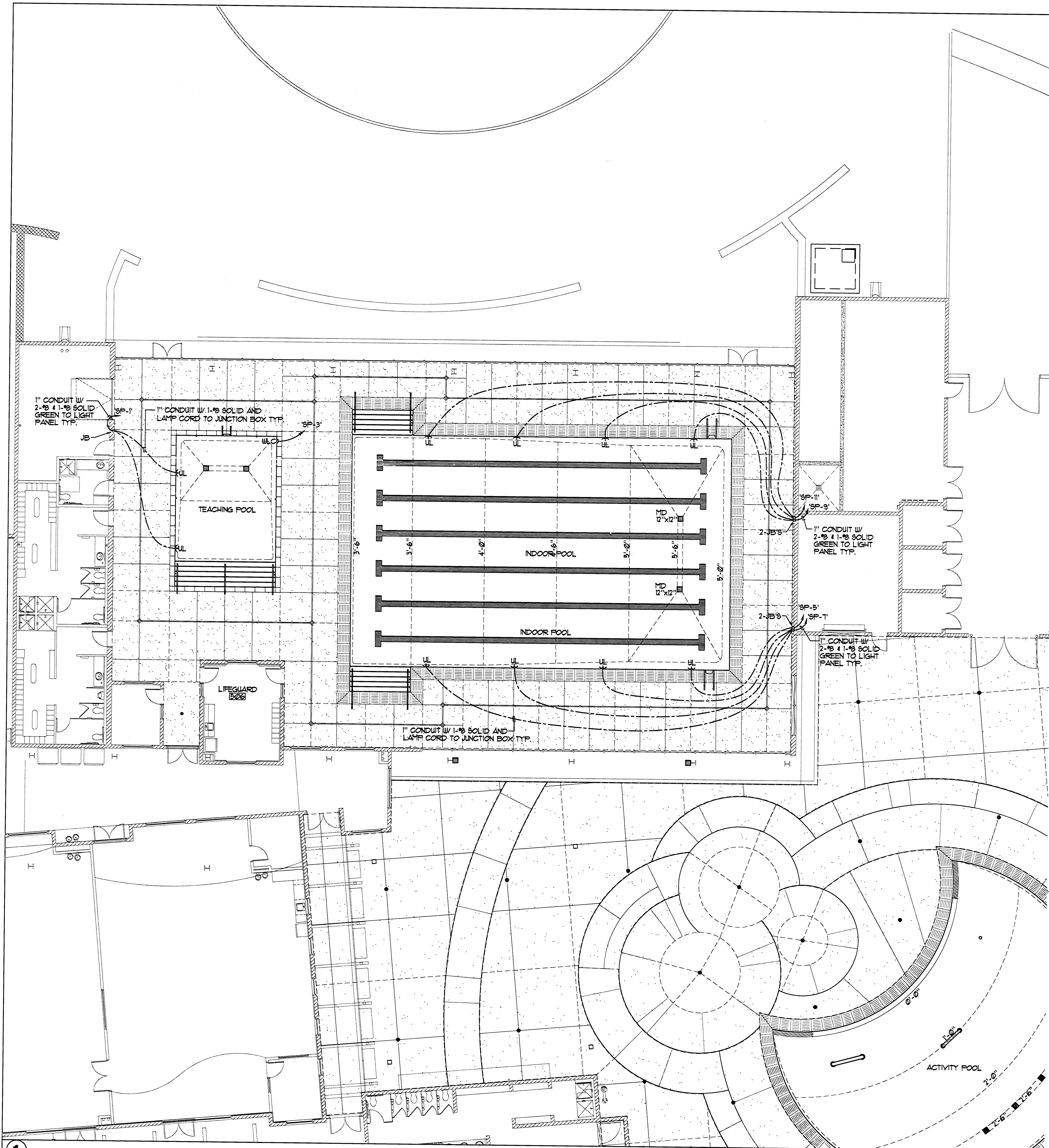
TEACHING / INDOOR POOL UNDERATER LIGHT PLAN 1/8"=1'-0"
