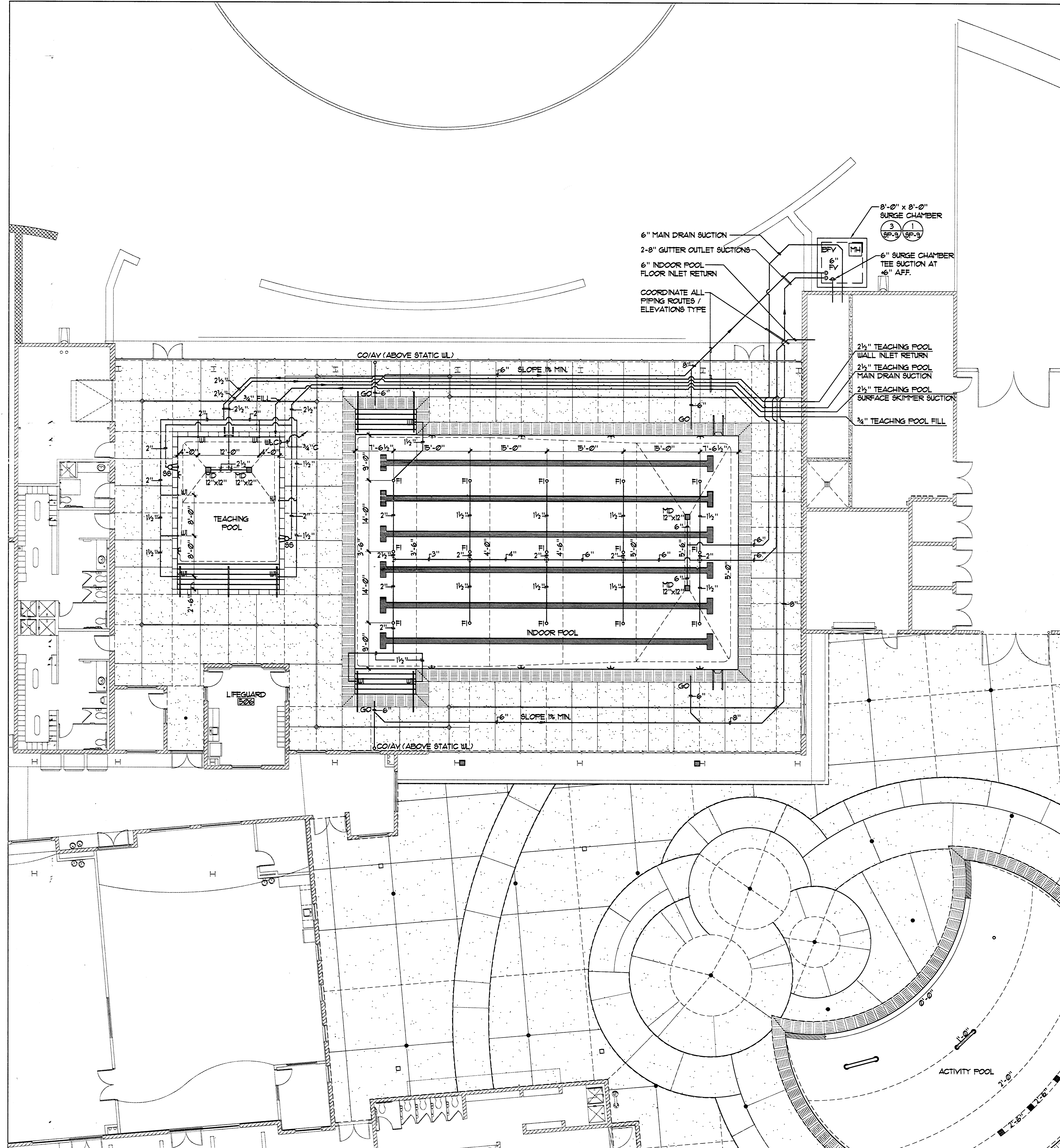
TEACHING / INDOOR POOL PIPING PLAN 1/8" = 1'-0"
