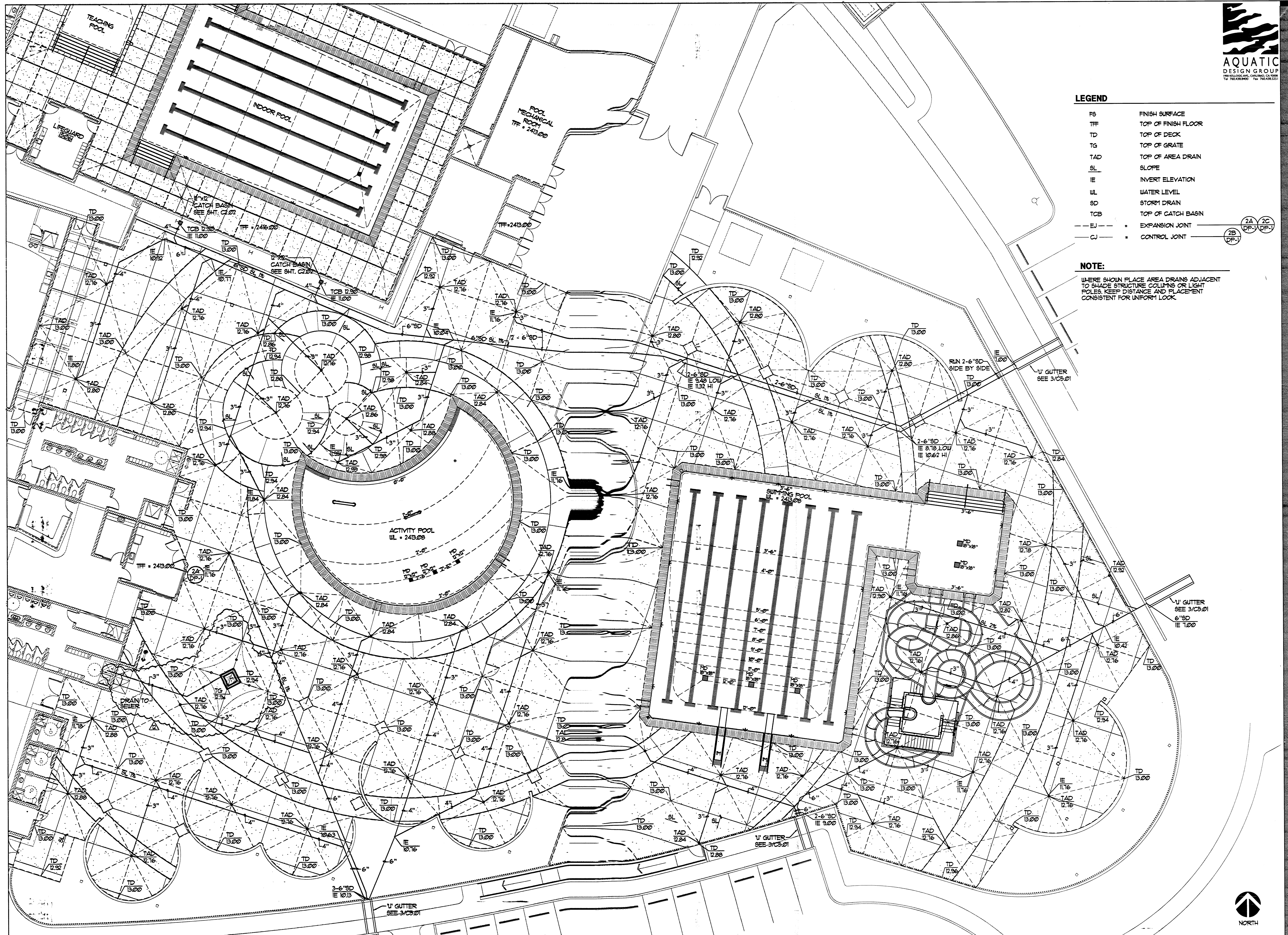
1 ACTIVITY/SWIMMING POOL DECK PLAN (VERTICAL CONTROL) 1"=10'-0"
