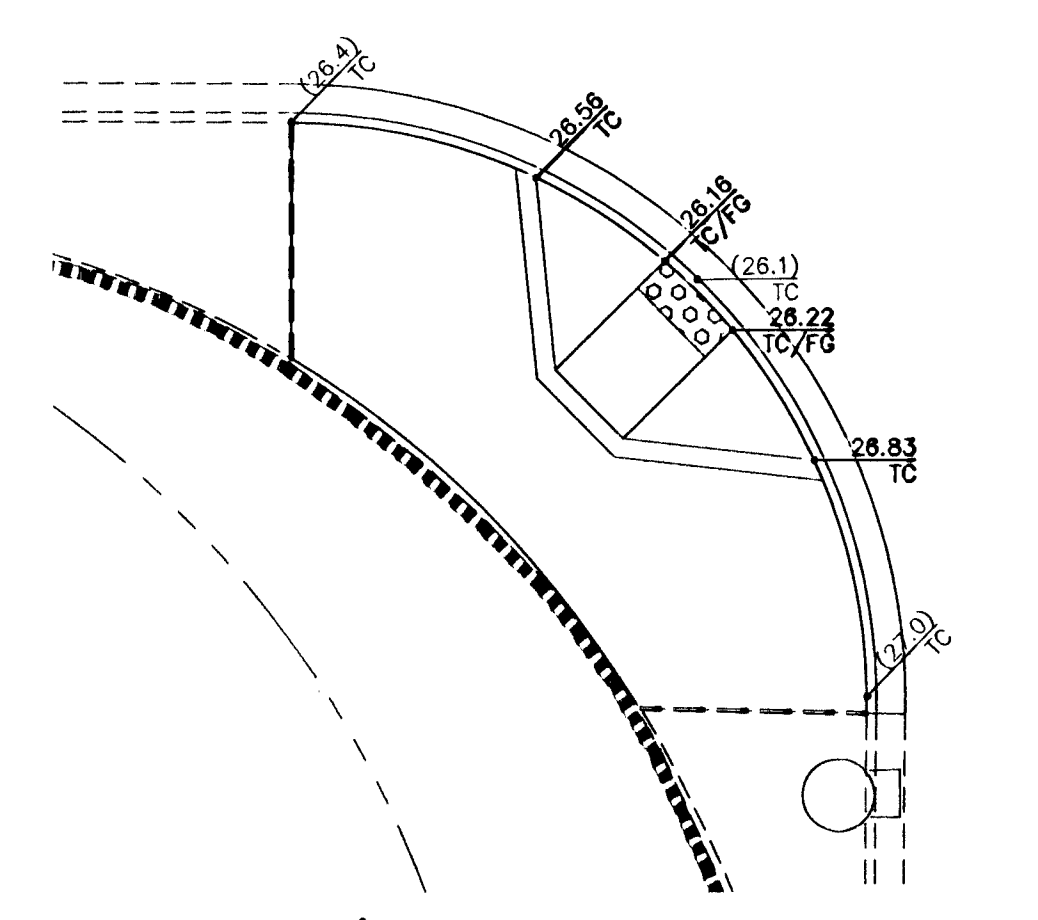
BONNEVILLE/MAIN INTERSECTION GRADING 1"=10'
