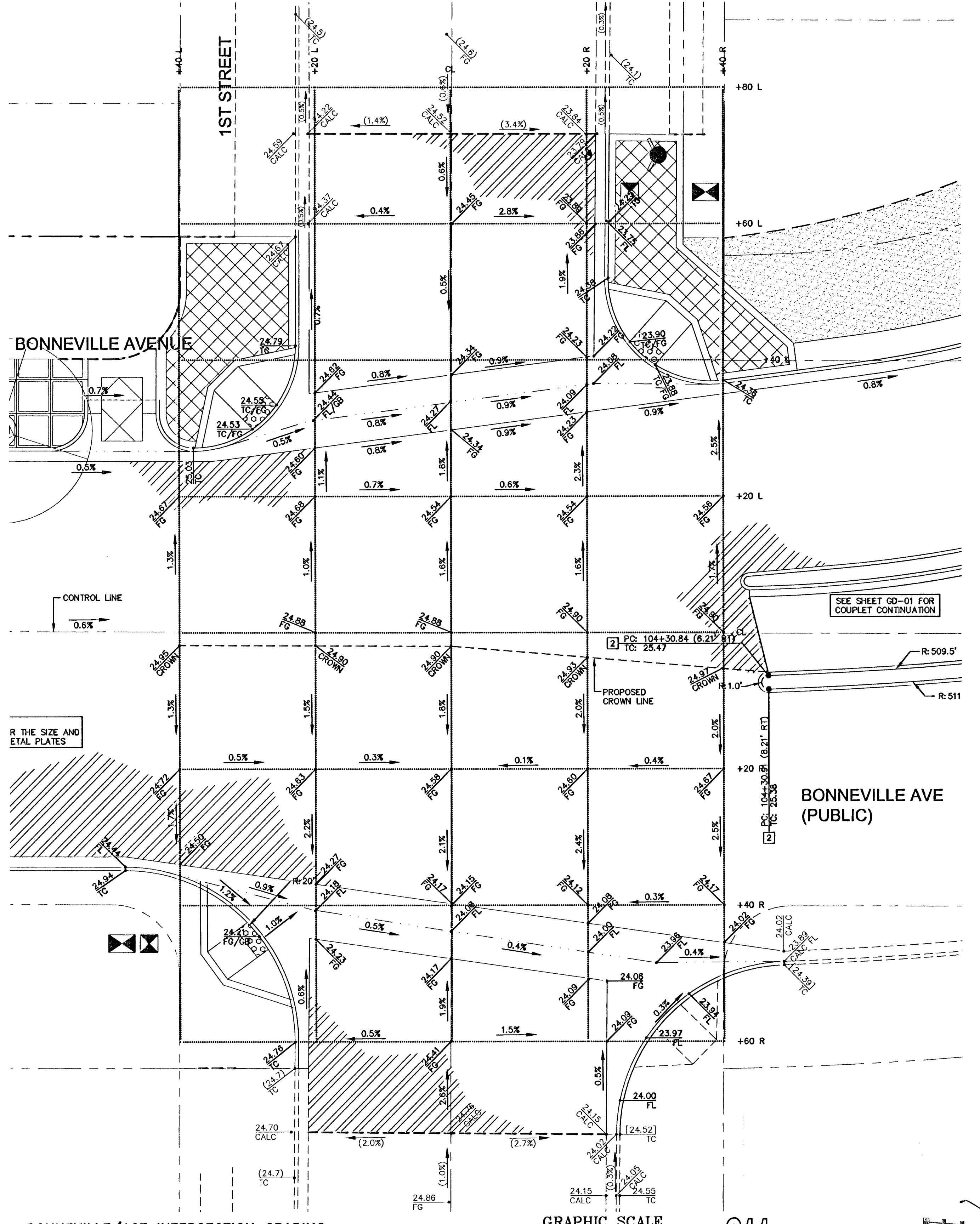
BONNEVILLE/1ST INTERSECTION GRADING 1"=10'
